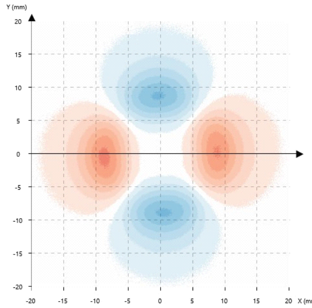
径向4极圆环
